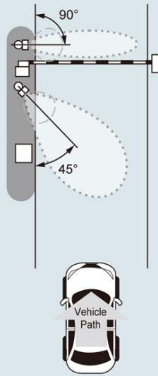
Barrier Gate
